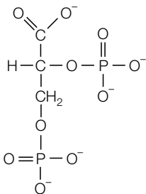
Fig. 4. 2,3-Bisphosphoglycerate.
