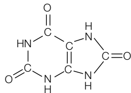
Fig. 6. Uric acid.
