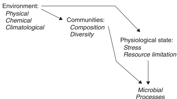
FIGURE 18.1 Linkages between environmental factors, microbial community composition, physiological state, and process dynamics.
