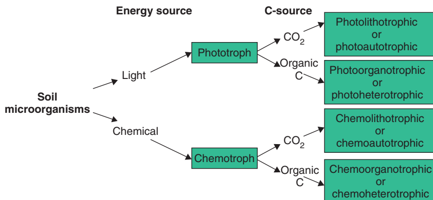
FIGURE 5.7 Physiological classification of soil bacteria in terms of their C and energy source (lithotrophs and organotrophs).
