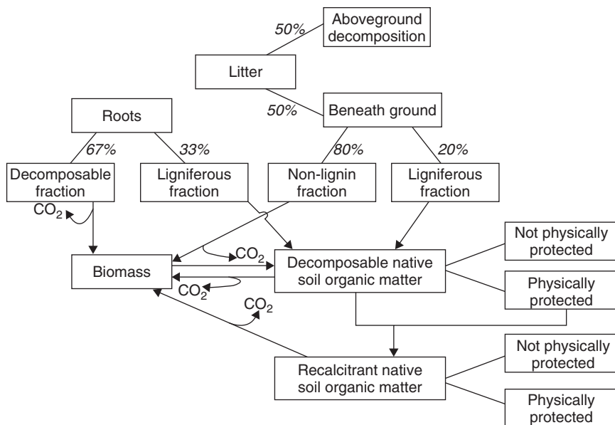
FIGURE 16.5 The structure of the Van Veen and Paul model for soil organic matter dynamics (with permission from Van Veen and Paul, 1981).
