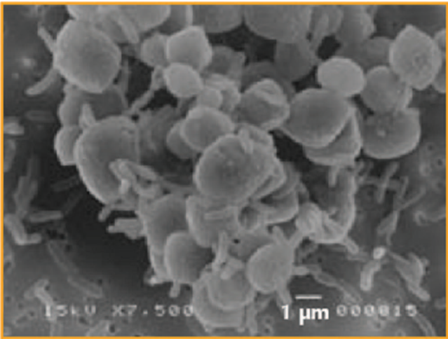
FIGURE 17.4 Geobacter sulfurreducens is the dominant metal-reducing microorganism isolated from subsurface environments and aquifers. It oxidizes aromatic hydrocarbons with Fe(III) as the electron acceptor. It can also oxidize organic pollutants while reducing other metals such as Mn(IV), U(VI), Te(VII), Co(VI), and Au(III). (Image courtesy of D. Lovely, University of Massachusetts. Reproduced from Anonymous (2003).)
