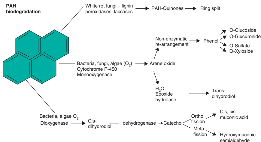
FIGURE 5.10 Schematic of soil microbial metabolism of polyaromatic hydrocarbons.
