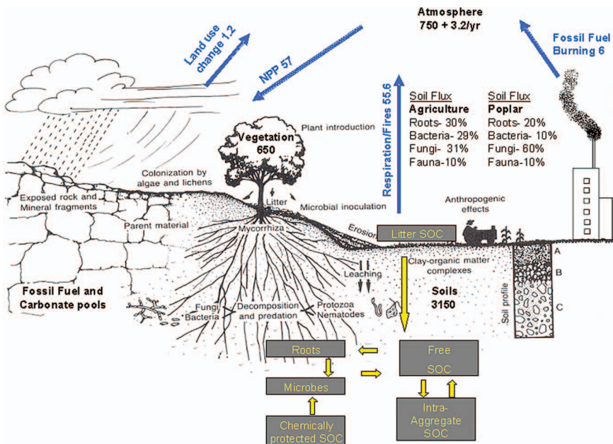
FIGURE 8.4 The global carbon cycle modified from Paul and Clark (1996). Pool and flux values modified from Gruber et al. (2004), which included preindustrial values for ecosystem C exchange, are in Pg-C for pools and Pg-C/y for fluxes. Flux values for the global C cycle when summed have failed to account adequately for an increase in atmospheric C of only 3.2 \text{ Pg-C/y} due in part to high error associated with measured values and poor understanding of all C source/sink mechanisms. The soil fluxes are driven largely by microbial participants, which researchers are currently working to quantify.
