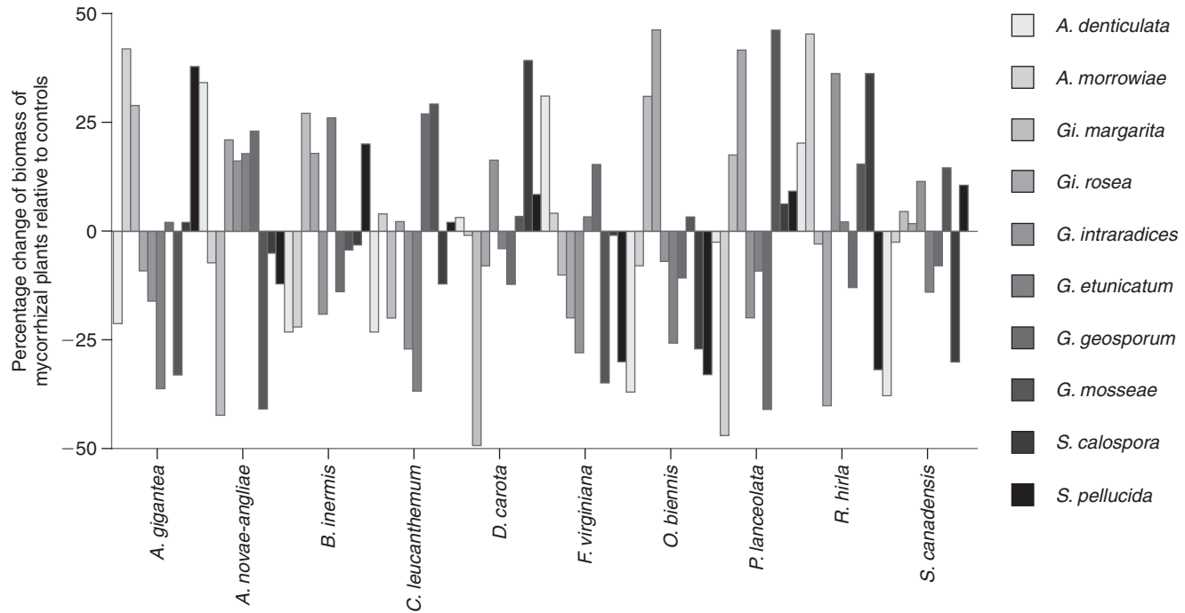
FIGURE 10.5 The influence of different species of arbuscular mycorrhizal fungi isolated from the Long-Term Mycorrhizal Research Site (LTMR; Guelph, ON, Canada) on the growth of different plant species, relative to nonmycorrhizal controls. Plant seeds used in this experiment were also collected from the LTMR. Plant responses to inoculation with the different fungal species ranged from highly positive to highly negative. Plant genera, from left to right along the horizontal axis, are Agrostis , Aster , Bromus , Chrysanthemum , Daucus , Fragaria , Oenothera , Plantago , Rudbeckia , and Solidago . Fungal genera, in the legend, are A. , Acaulospora ; Gi. , Gigaspora ; G. , Glomus ; S. , Scutellospora . For all treatments, the 95% confidence interval is \pm 18\% . (Reprinted from Klironomos, 2003, with permission; copyright 2003, Ecological Society of America.)
