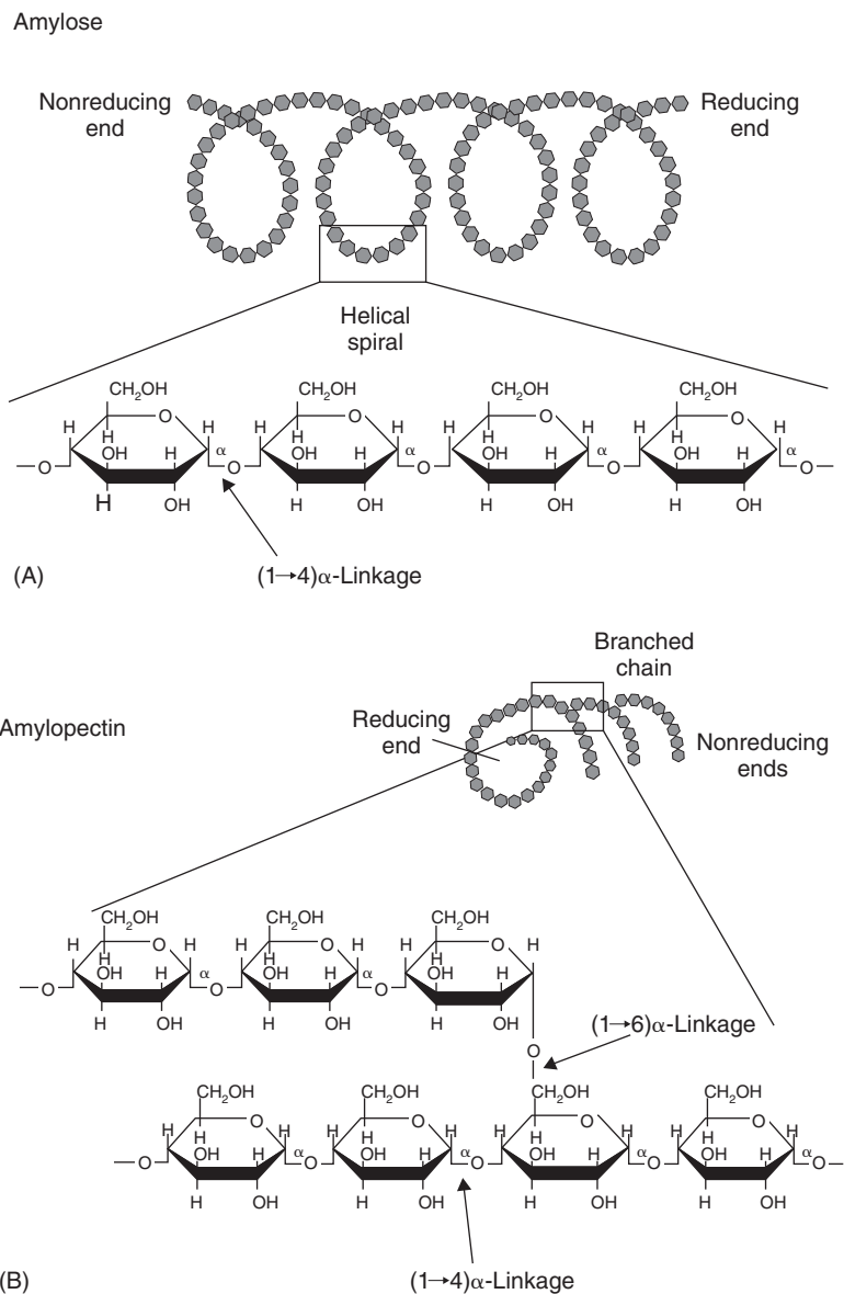
FIGURE 12.7 The structure of starch showing the (A) \alpha(1-4) linkage of amylose and (B) \alpha(1-6) branched linkage of amylopectin.
