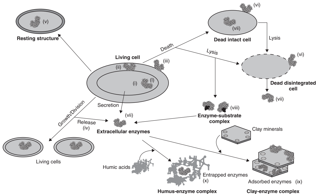
FIGURE 3.4 Locations of enzymes (from Burns, 1982, adapted by Klose, 2003). (i) Intracellular enzymes. (ii) Periplasmatic enzymes. (iii) Enzymes attached to outer surface of cell membranes. (iv) Enzymes released during cell growth and division. (v) Enzymes within nonproliferating cells (spores, cysts, seeds, endospores). (vi) Enzymes attached to dead cells and cell debris. (vii) Enzymes leaking from intact cells or released from lysed cells. (viii) Enzymes temporarily associated in enzyme– substrate complexes. (ix) Enzymes absorbed to surfaces of clay minerals. (x) Enzymes complexed with humic colloids. (Reproduced with permission from Taylor & Francis Group, LLC.)
