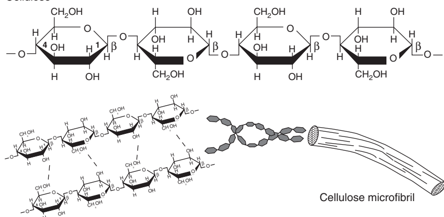
FIGURE 12.8 Cellulose structure showing \beta(1-4) linkages combining glucose residues into a single chain polymer. Chains are cross-linked by hydrogen bonds to form cellulose microfibrils.
