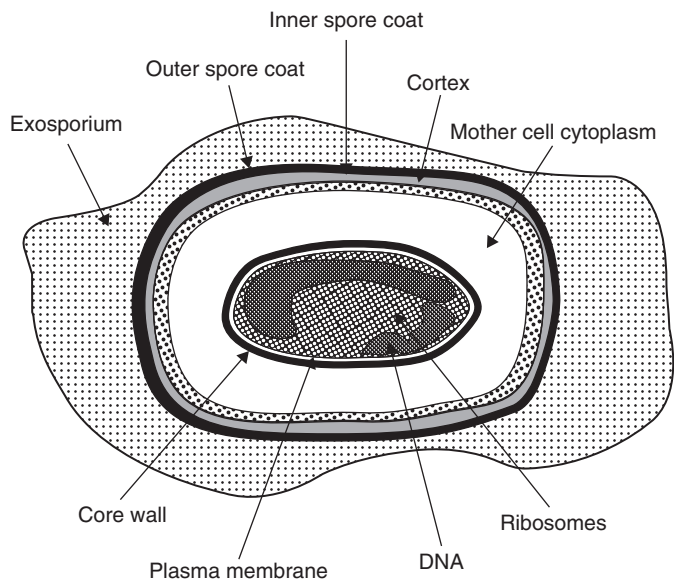
FIGURE 5.4 Major characteristics of a bacterial spore.
