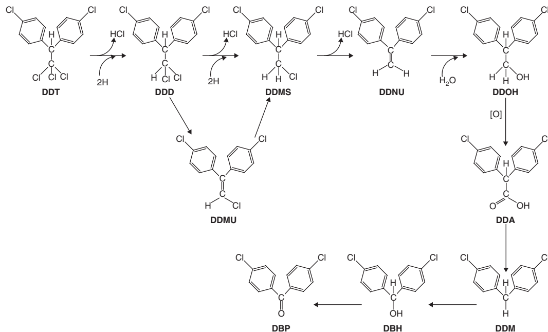
FIGURE 17.3 Proposed pathway for bacterial metabolism of DDT via reductive dechlorination. DDT, 1,1,1-trichloro-2,2-bis( p -chlorophenyl)ethane; DDD, 1,1-dichloro-2,2-bis( p -chlorophenyl)ethane; DDMU, 1-chloro-2,2-bis( p -chlorophenyl)ethylene; DDMS, 1-chloro-2,2-bis( p -chlorophenyl)ethane; DDNU, 2,2-bis( p -chlorophenyl)ethylene; DDOH, 2,2-bis( p -chlorophenyl)ethanol; DDA, bis( p -chlorophenyl)acetic acid; DDM, bis( p -chlorophenyl)methane; DBH, 4,4'-dichlorobenzhyrol; and DBP, 4,4'-dichlorobenzophenone (with permission from Aislabie et al. , 1997).
